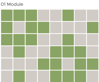
MINI-SQR-20 Module : 254x254mm / 0.69 sq. ft. Gap : 2mm | Chip Size : 30x30mm
